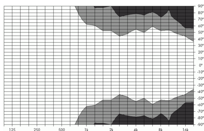
Isobar diagram horizontal and vertical
