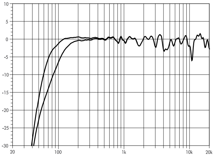
8S frequency response, standard and CUT modes
