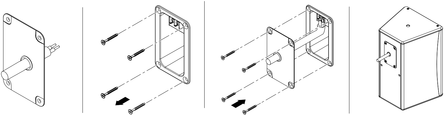
Installing the fixed cable connection
