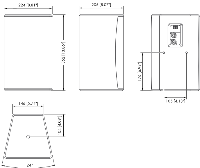
8S cabinet dimensions in mm [inch]
