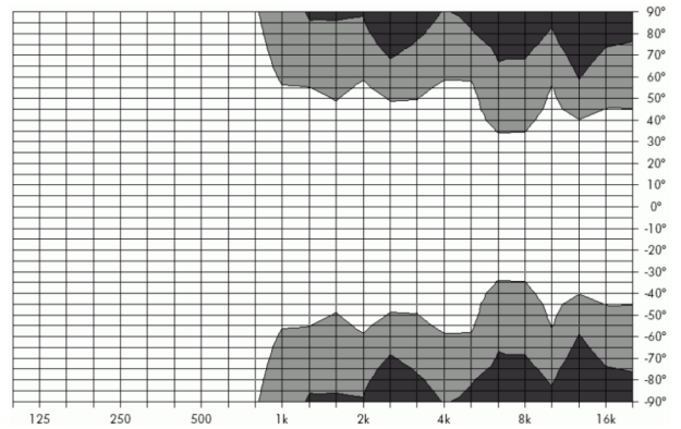
Fig. 12: Isobar diagram vertical
