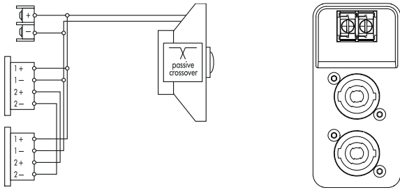
Fig. 3: Connector wiring
