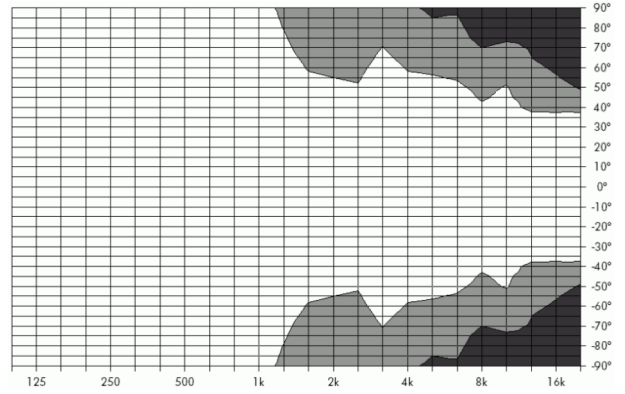
Fig. 10: Isobar diagram vertical
