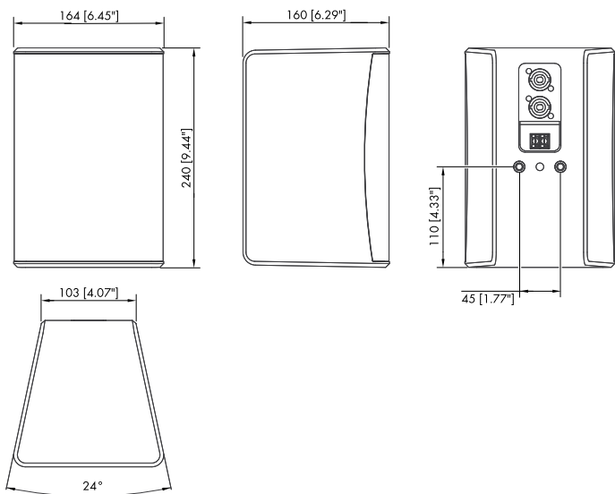
Fig. 16: 5S cabinet dimensions in mm [inch]
