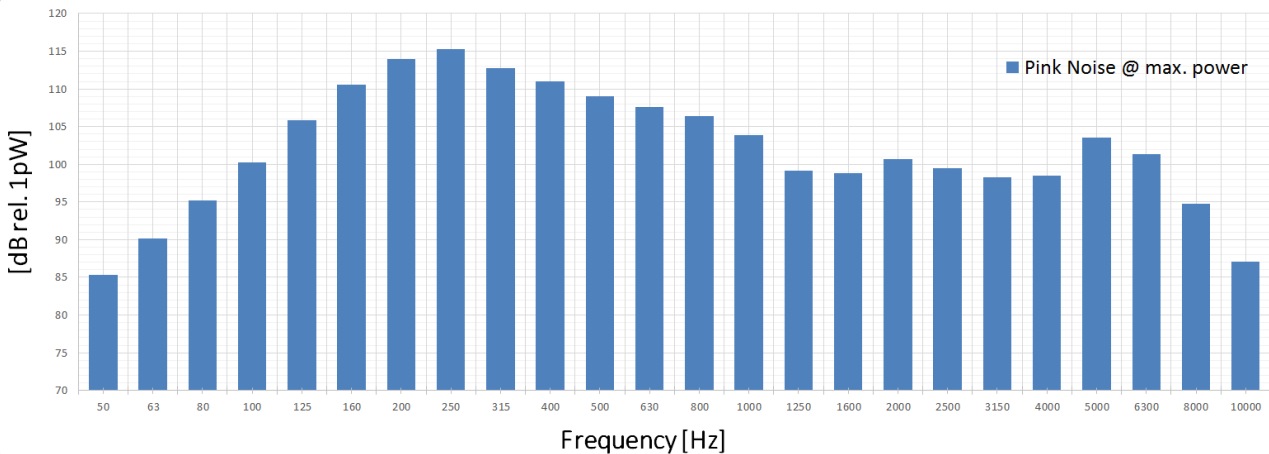
DS3 frequency response @ PA3 setting 'Pink' (maximum sound power)
