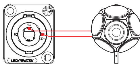
2-wire connection, e.g. with DS2 (PA3 in bridge mode)
