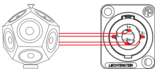
4-wire connection for DS3 loudspeaker
