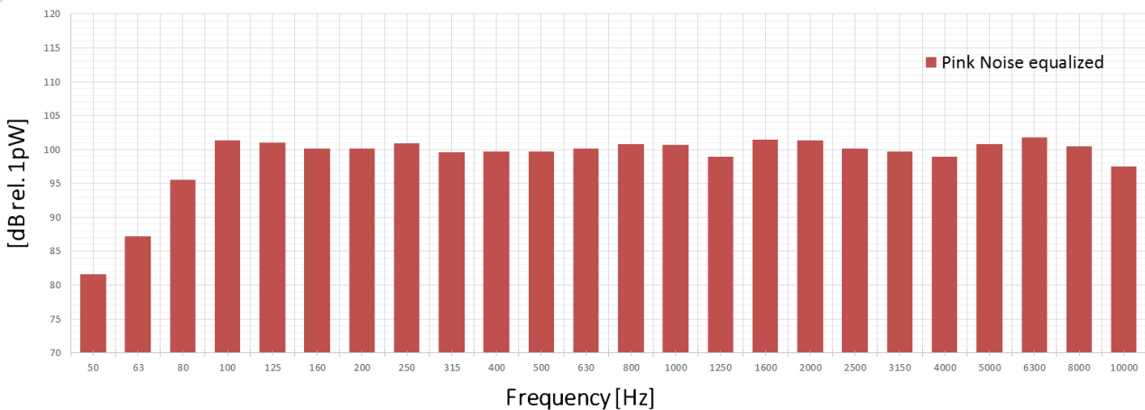
DS3 frequency response @ PA3 setting 'EQ Pink' (equalized)
